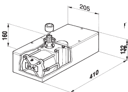
750 drive unit & foundation box
